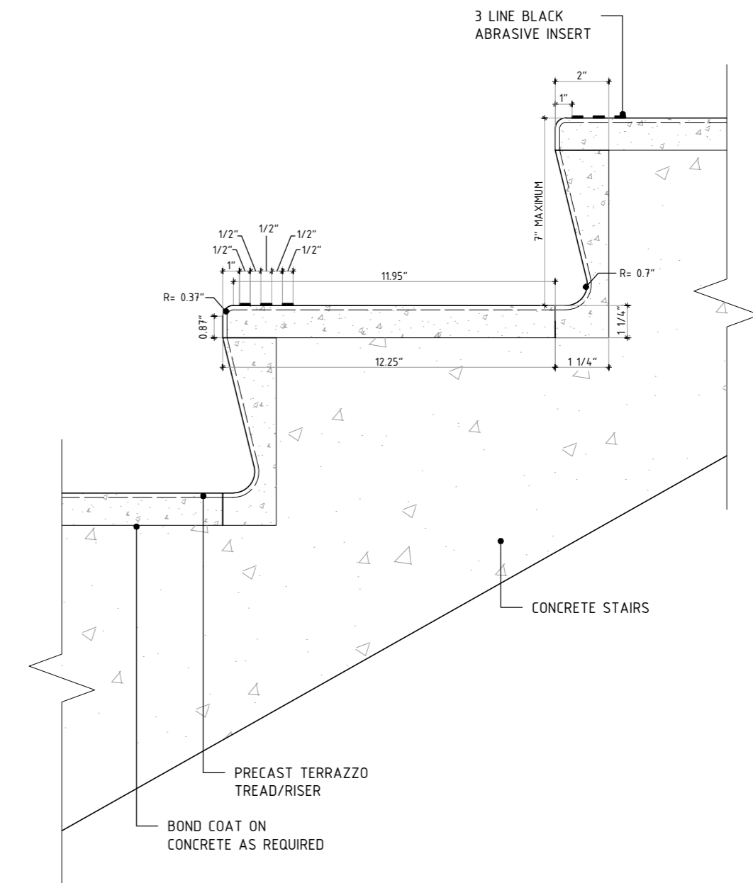
C1 STAIR DETAIL
